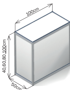
15. System platform reinforced 100 x 50 h=40/60/80/100
