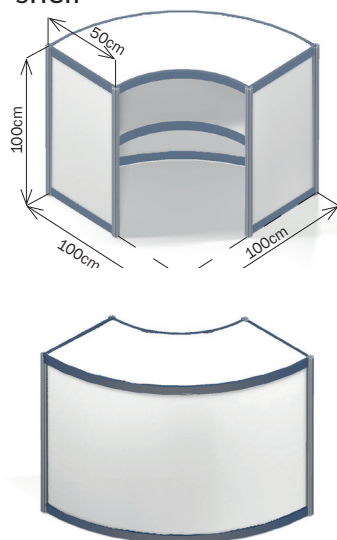
12. Curved counter with shelf
