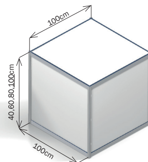
16. System platform reinforced 100 x 100 h=40/60/80/100
