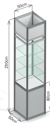
19. Glass display case, 3 shelves 50 x 50 h=250
